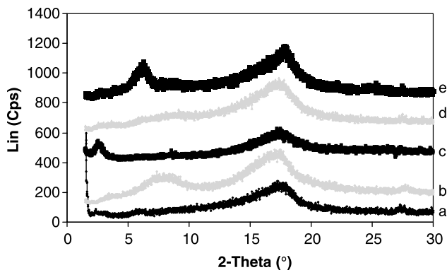
Fig. 8. X-ray diffraction patterns for (a) Nafion ® membranes and Nafion ® membranes filled with 3 wt% of (b) Native MMT, (c) Cloisite 30B, (d) Cloisite BHB and (e) Cloisite ACA.
