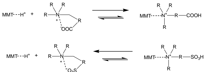
Fig. 5. Equilibrium of cation exchange between \text{H}^+ -MMT and acid containing ammonium cations.
